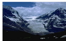
Athabasca Glacier
